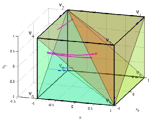
Fig. 3. The Delaunay triangulation of the cube used in Example 2, and some simulated trajectories of the closed-loop system.
